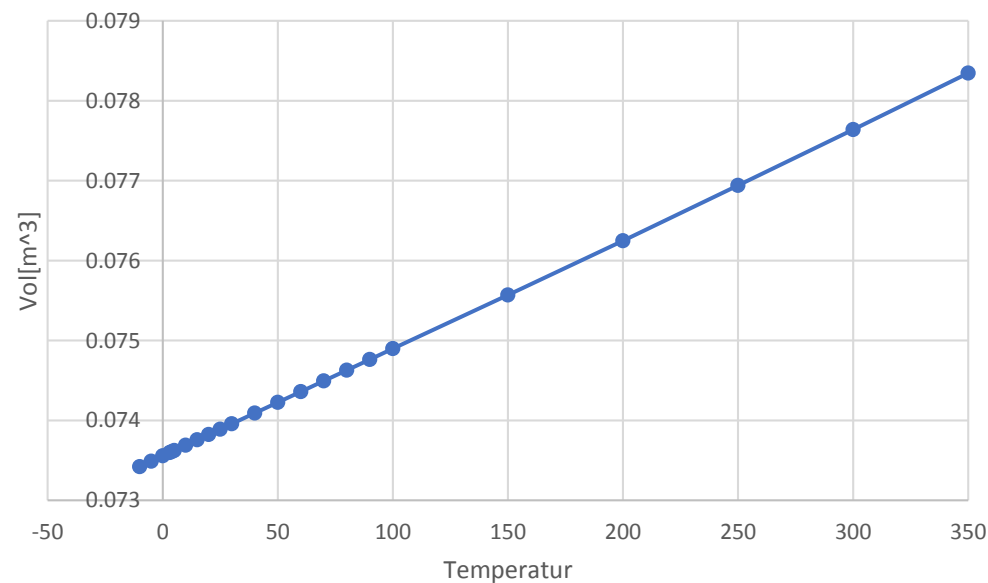
1 t Quecksilber: Vol[m 3 ] vs Temp[C]
