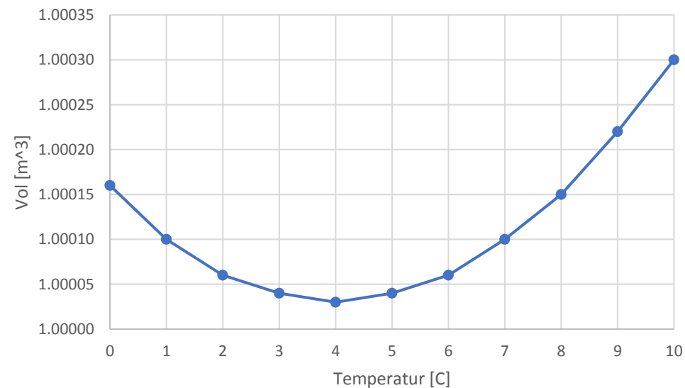
1 t Wasser: Vol[m 3 ] vs Temp[C]
