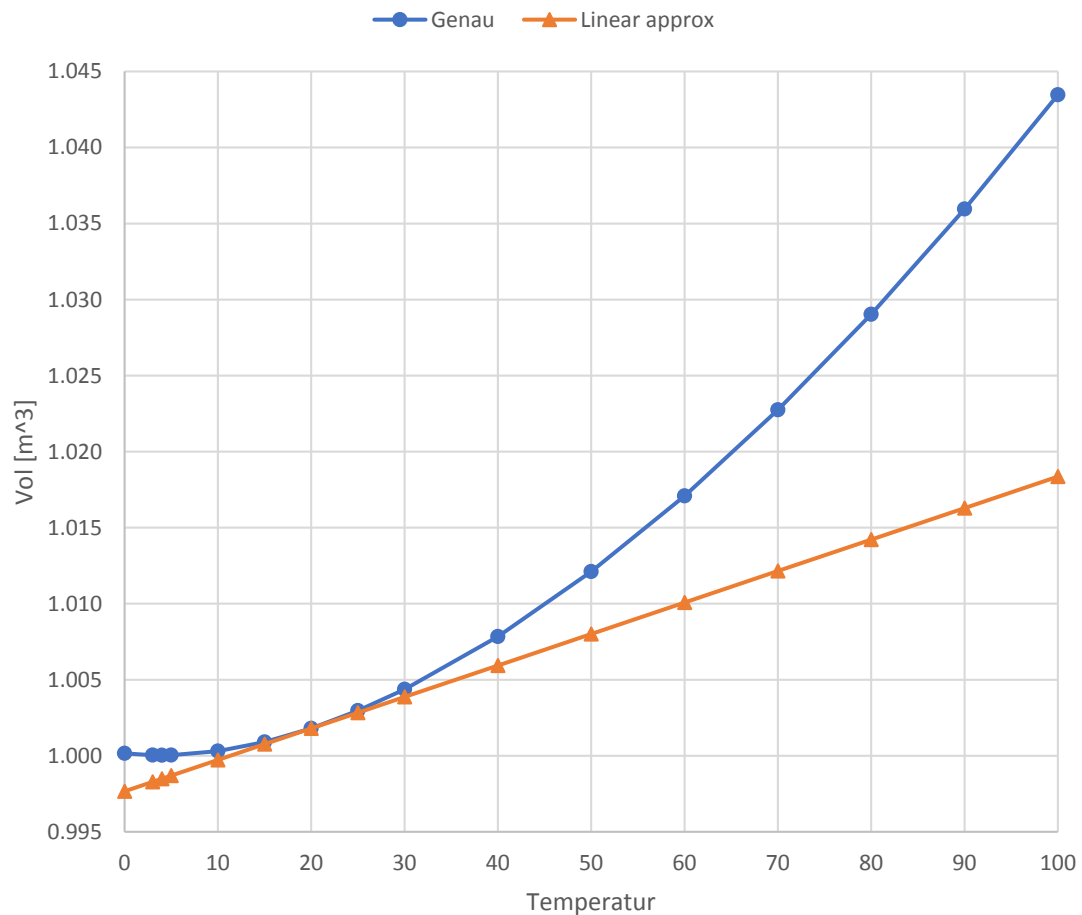
1 t Wasser: Vol[m 3 ] vs Temp[C]
