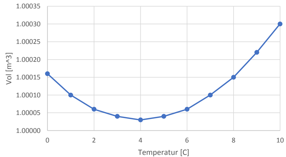
1 t Wasser: Vol[m 3 ] vs Temp[C]
