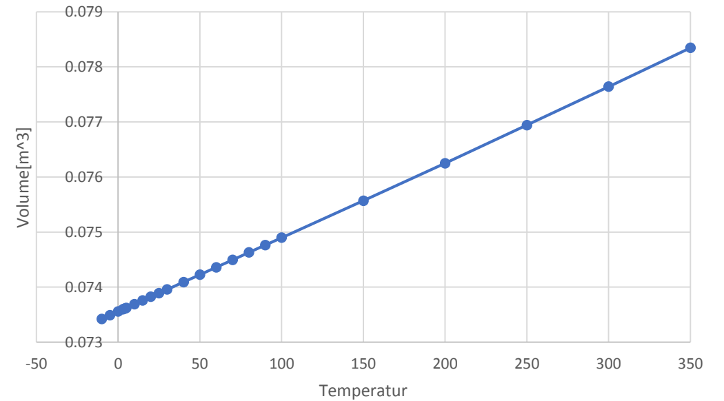
1 t Quecksilber: Vol[m 3 ] vs Temp[C]
