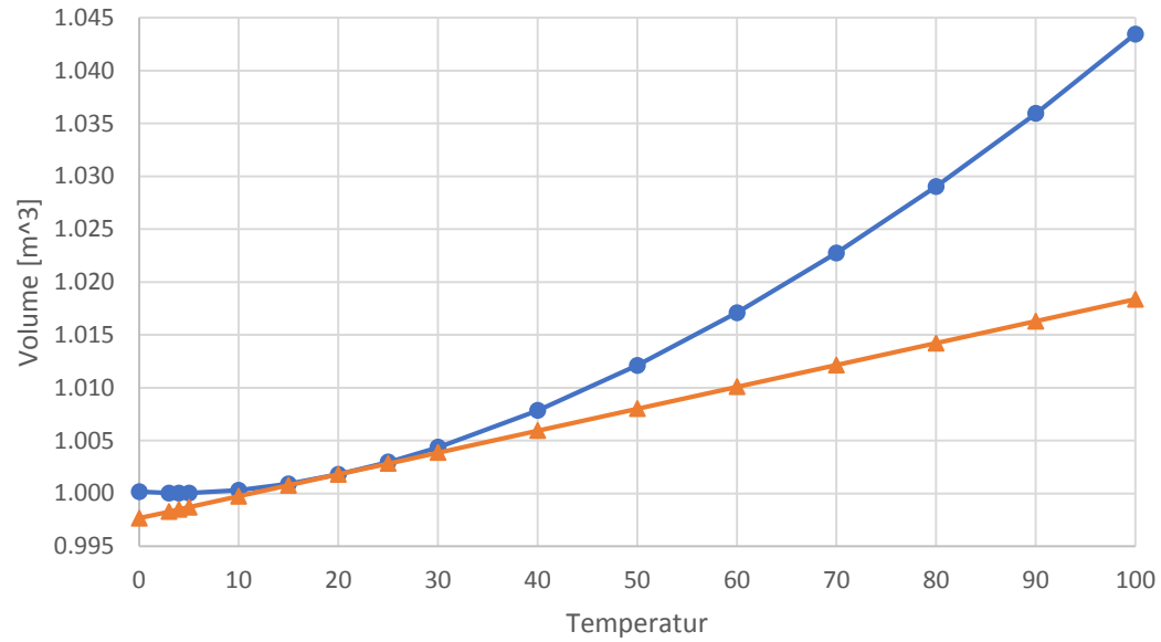
1 t Wasser: Vol[m 3 ] vs Temp[C]
